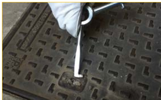
Configuration 2: L - shaped end for scraping in the inside of the slot and release the rotation for opening the lid.
